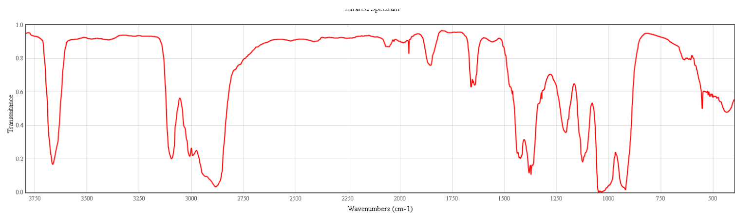
IR-A5 C 3 H 6 O (gas phase spectrum)
